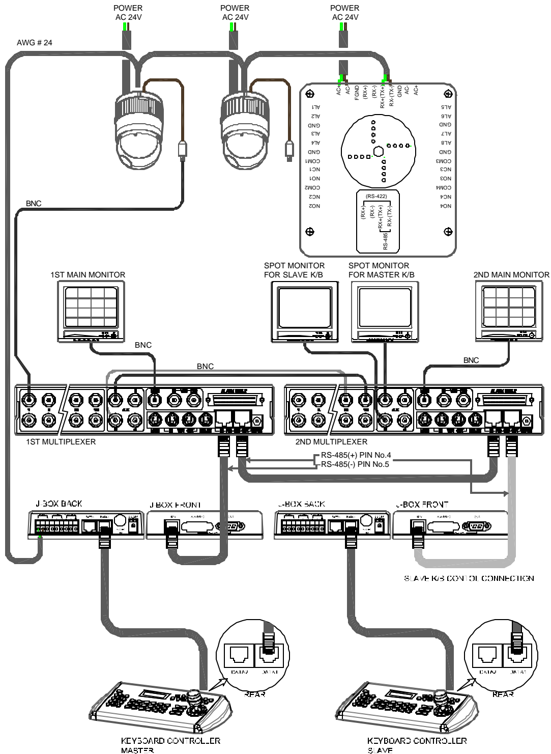
Figure 5 – Two Multiplexer with Slave Keyboard Controller
