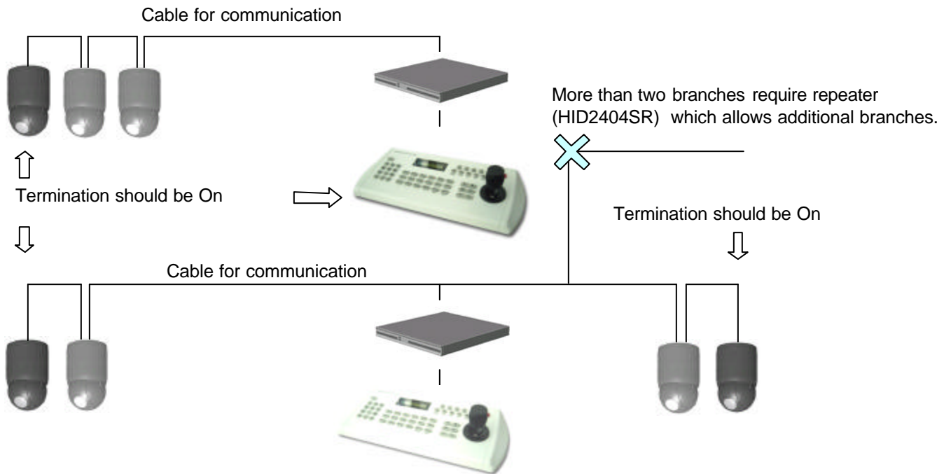
Figure 7 – Termination and ID Switches.
