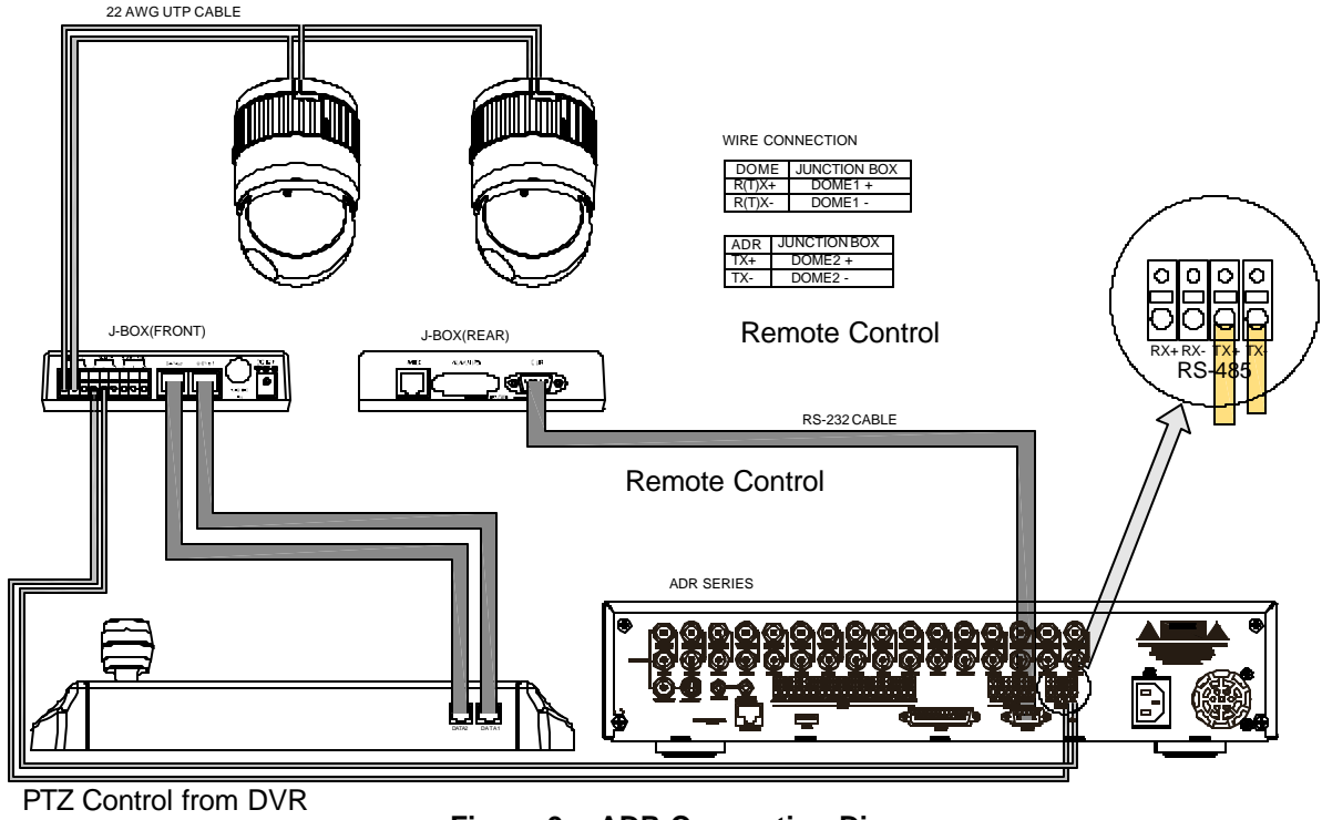
Figure 9 – ADR Connection Diagram
